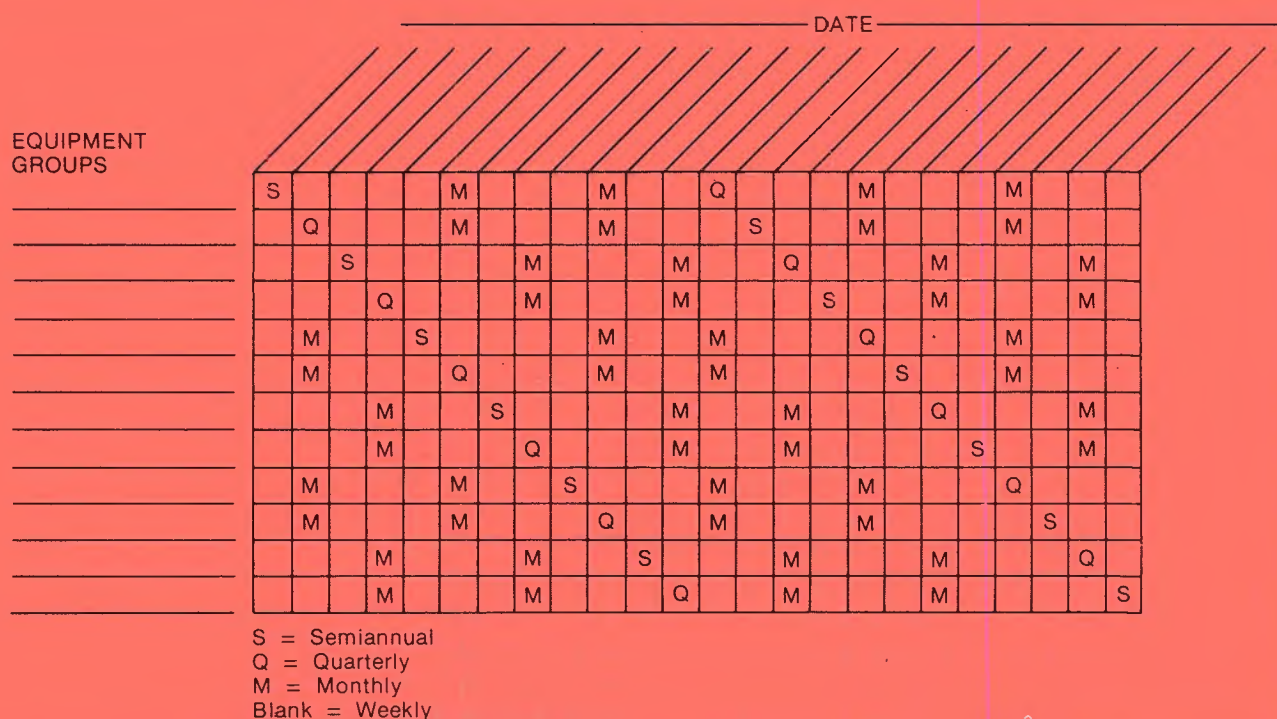
Figure 1 Progressive maintenance format. Cycles rotate through 12 equipment groups in 24 weeks.
