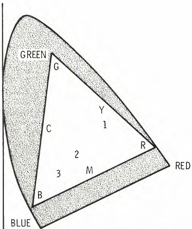
Figure 1 Standard color TV phosphors will reproduce most colors within the inside triangle. However, the highly saturated colors which would fall in the shaded portions of this chromaticity diagram cannot be accurately reproduced by television, even though they can be perceived by the eye. The numbers represent "white light" standards.
