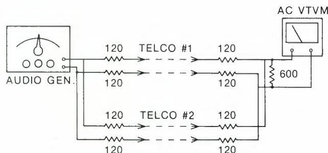
Figure 1 If you have a spare telco loop of equal quality to your main, you can check the phasing to see if they will be satisfactory as a stereo pair by doing the following simple test. First, connect the equipment as shown above and send a 1 kHz signal at normal program level down the lines. If the lines are totally out of phase, the meter at the receive end will read nearly zero. If that happens, reverse the connections to one of the pairs at either end and try again. When the pairs are in proper static phasing, the meter will indicate the audio generator output level minus the line losses and 6 dB for the splitter and adder networks. Next, mark the connections so that they can always be connected in proper phase. Now vary the frequency of the audio generator across the audio band and record the response across the 600-ohm resistor. Assuming that the lines have flat response, the phasing is satisfactory up to the frequency where the response begins to roll off. If you're not sure of the lines, record the response of each line individually into a 600-ohm load before phase testing.
