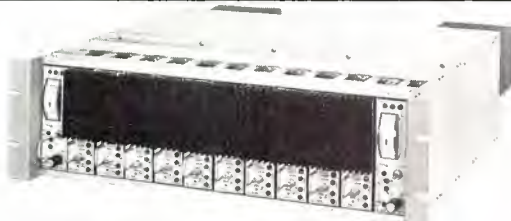
D-509 Audio Distribution Amplifier , 6 outputs, +30 dBm, up to ten D.A.'s with redundant common P.S. in 5 1/4" rack frame
